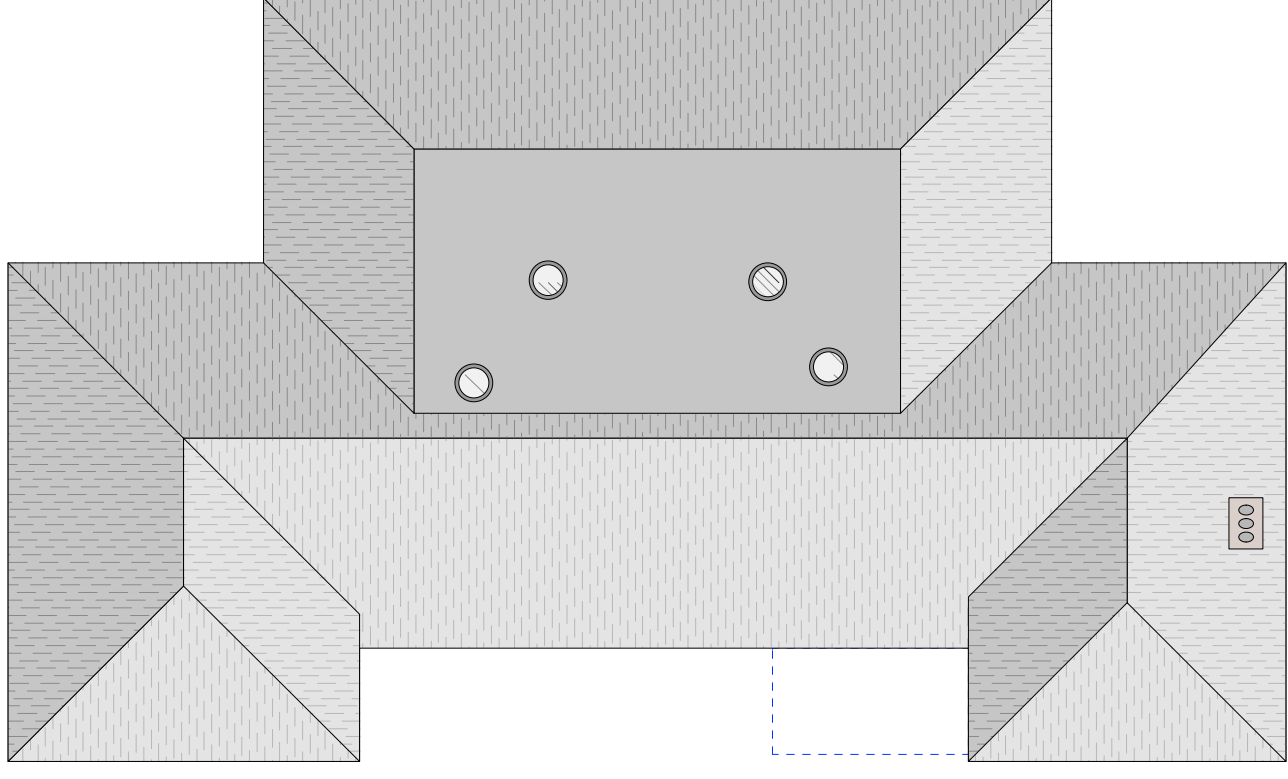
roof plan
